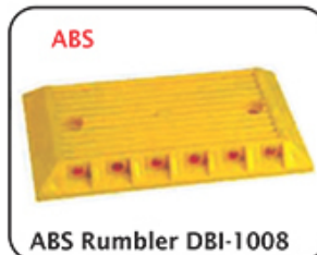
ABS Rumbler DBI-1008 250 x 150 x 32 mm with 6 + 6 Cat Eyes (Glass Beads)
